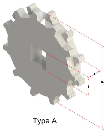
Machined Sprocket Dimensions
